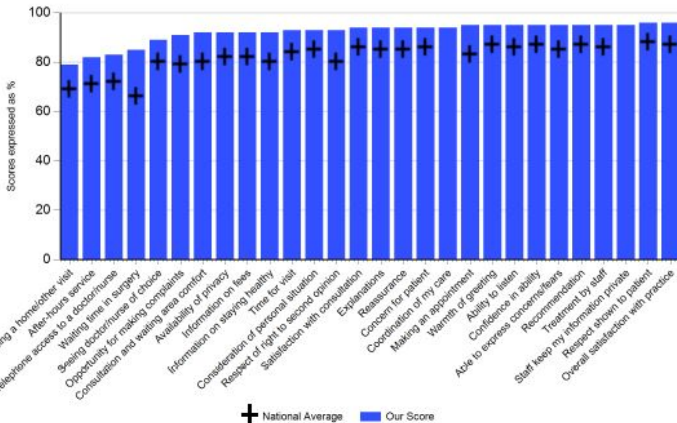
Overall scores
